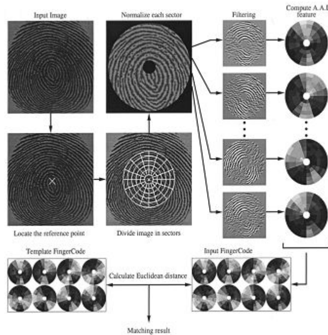
Fig. 5. System diagram of fingerprint authentication system[5]
